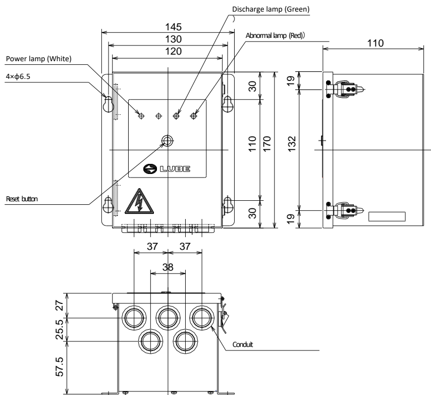
[Power Controller]
